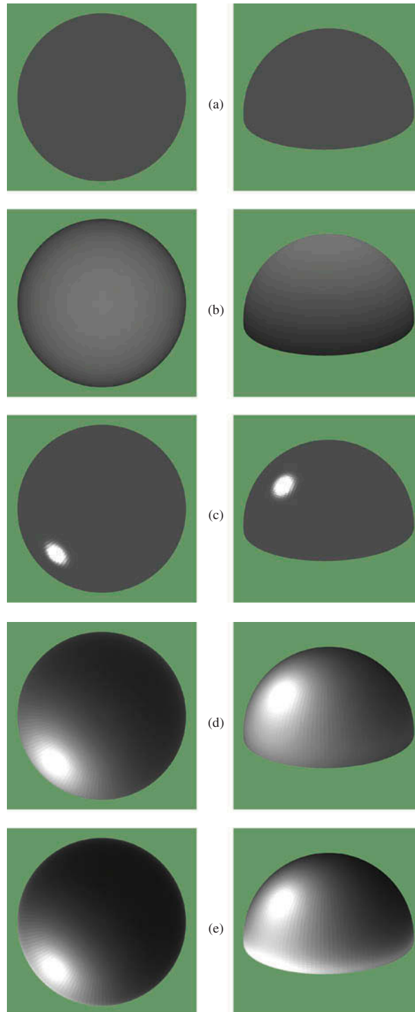
Figure 1. The radiance for (a) uniform, (b) overcast, (c) sharp, (d) clear, and (e) turbid skies. In the left column, the center of the circle corresponds to an inclination of 90^\circ and the circumference to an inclination of 0^\circ . In the right column, the radiance is shown on the side of a hemisphere, where each point represents one direction from the sky.
